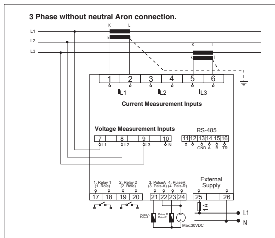
Figure 8: ARON connection (3 phase without neutral connection)
