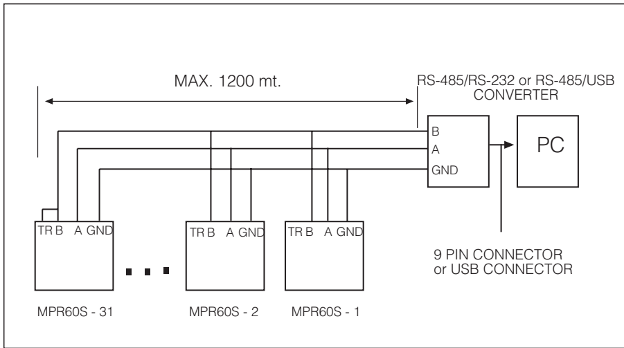
Figure 9: 31 devices can be connected to the same line.* * Max. 20 devices are advised to connect to the same line.
