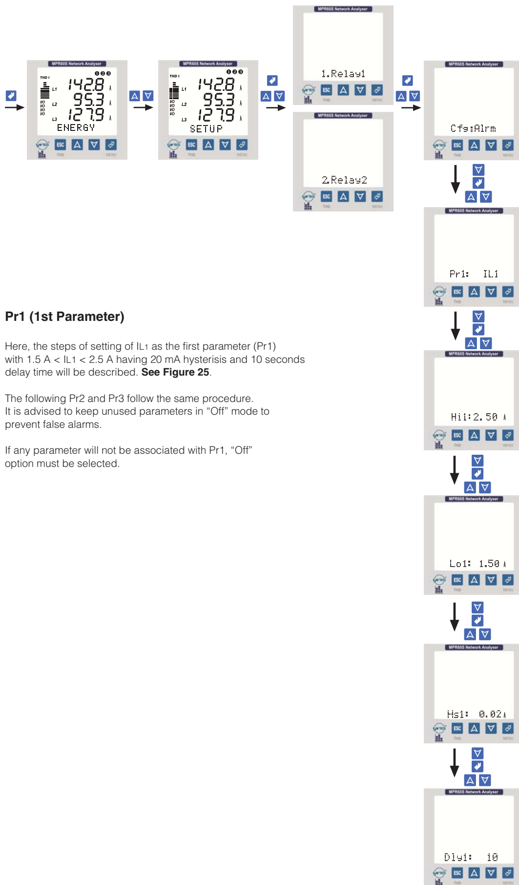
Figure 25: Setting of IL1 as the first parameter with 1.5 \text{ A} < \text{IL1} < 2.5 \text{ A} having 20 mA hysteresis and 10 seconds delay time.
